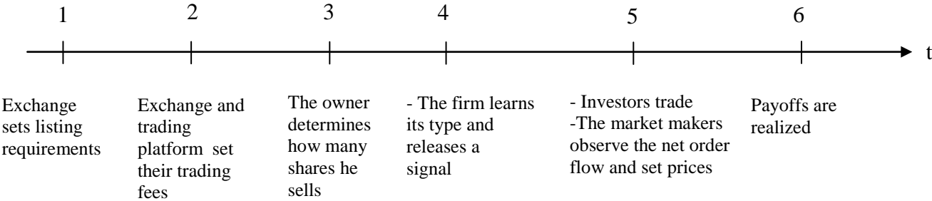
Figure 1: extensive form of the game
