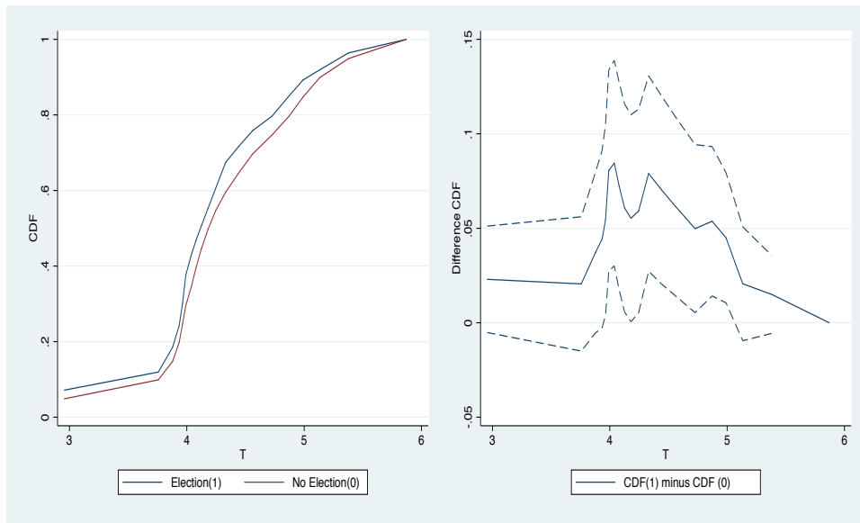
Figure 7 Cumulative Density Functions
