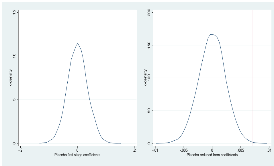
Figure A.4 Random permutation test
