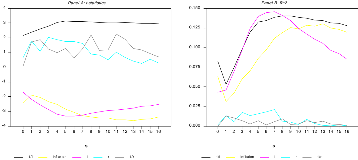
Figure 3: t -statistics and R^2 of univariate regressions of the forecast error \hat{\delta}_{t+1,t+1-\tau} on interest rates and gross-net interest rate ratios (both nominal and real) as well as inflation.
