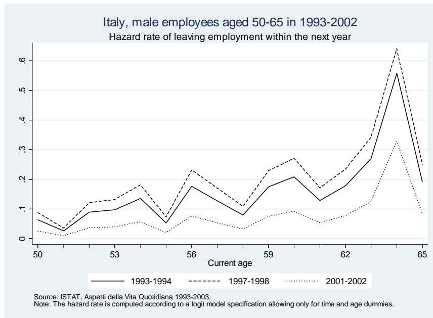
Figure 3: Age-profile of the hazard rate of exiting employment.
