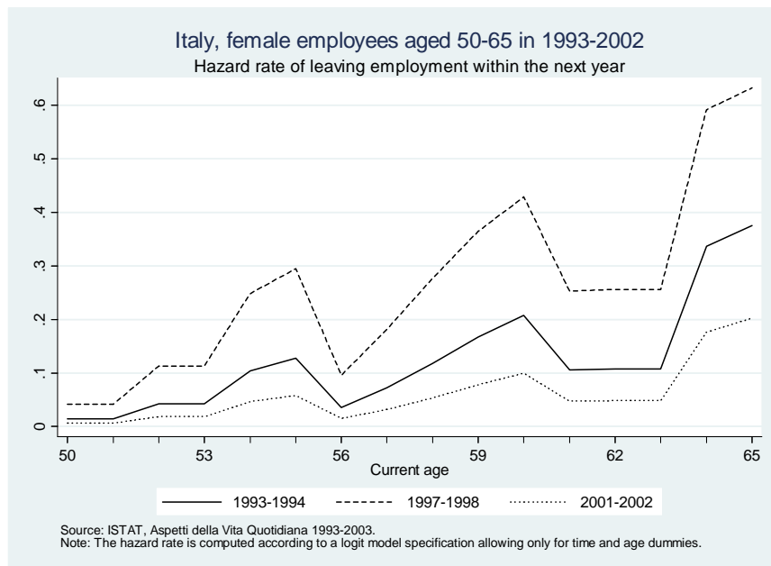
Figure 4: Age-profile of the hazard rate of exiting employment.
