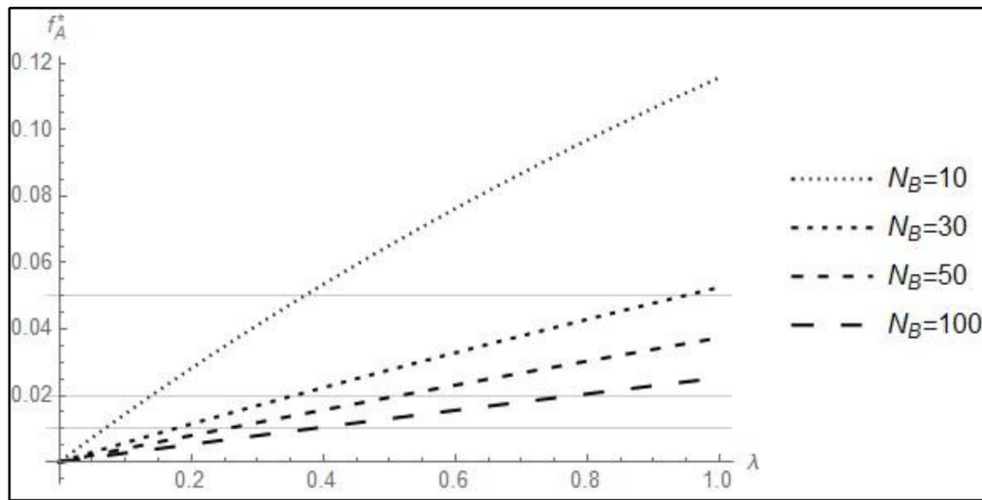
Figure 1: Equilibrium trading fee
